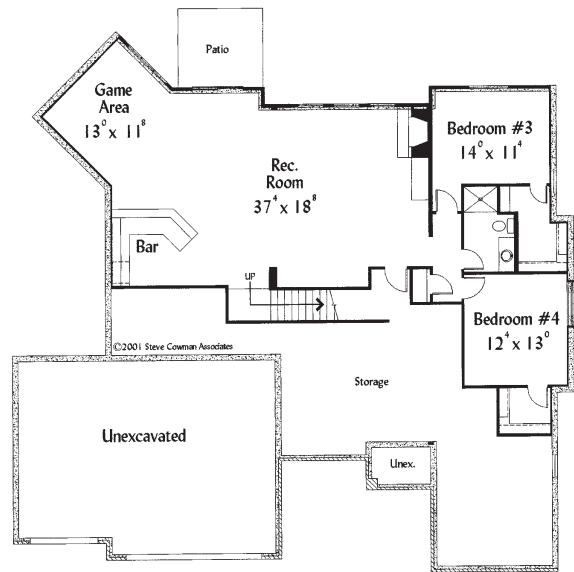
Optional Basement Finish Plan
